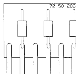
808577 DIODE PACK LOCATED UNDER DASH NEAR SWITCHES
